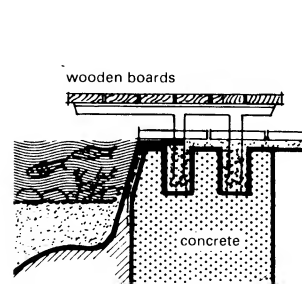
⑥ A cantilevered jetty
